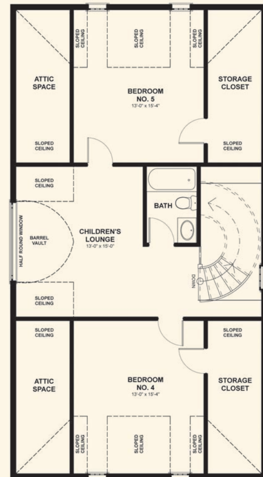
THREE STOREY – THIRD FLOOR
